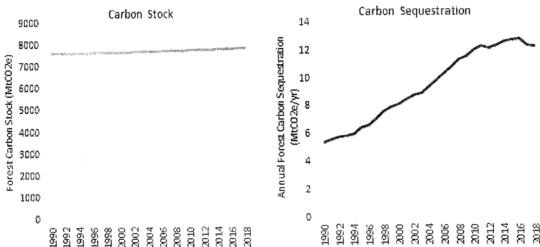
Figure 2. Maine Forest Sector Carbon Stock and Sequestration (MtCO 2 e) (Source: Daigneault, 2021).
