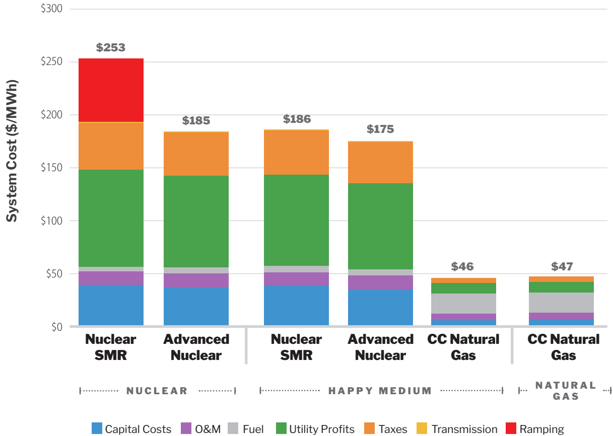
FIGURE 26. The Always On LCOE for each new resource in each scenario is shown in the chart above. Variations in cost between natural gas and nuclear are mostly driven by differences in utilization rates, or capacity factors, in the Natural Gas, Nuclear, and Happy Medium scenarios. Data from AOER's Always On LCOE model.
