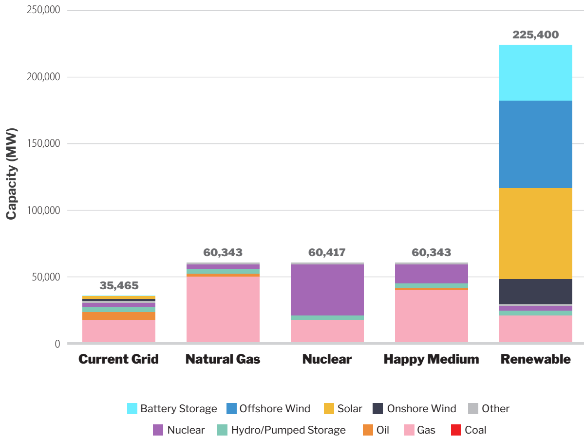
FIGURE 21. The Renewable scenario would require almost 6.4 times more installed capacity on the New England electric grid than is currently in service to maintain a reliable system, based on 2023 wind and solar output. This massive buildout of capacity would drive significant cost increases for families and businesses. Data from AOER’s capacity expansion model.
